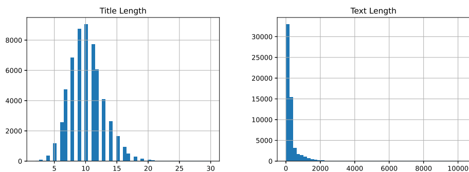
Figure 4: Distribution of number of words in titles and texts respectively
